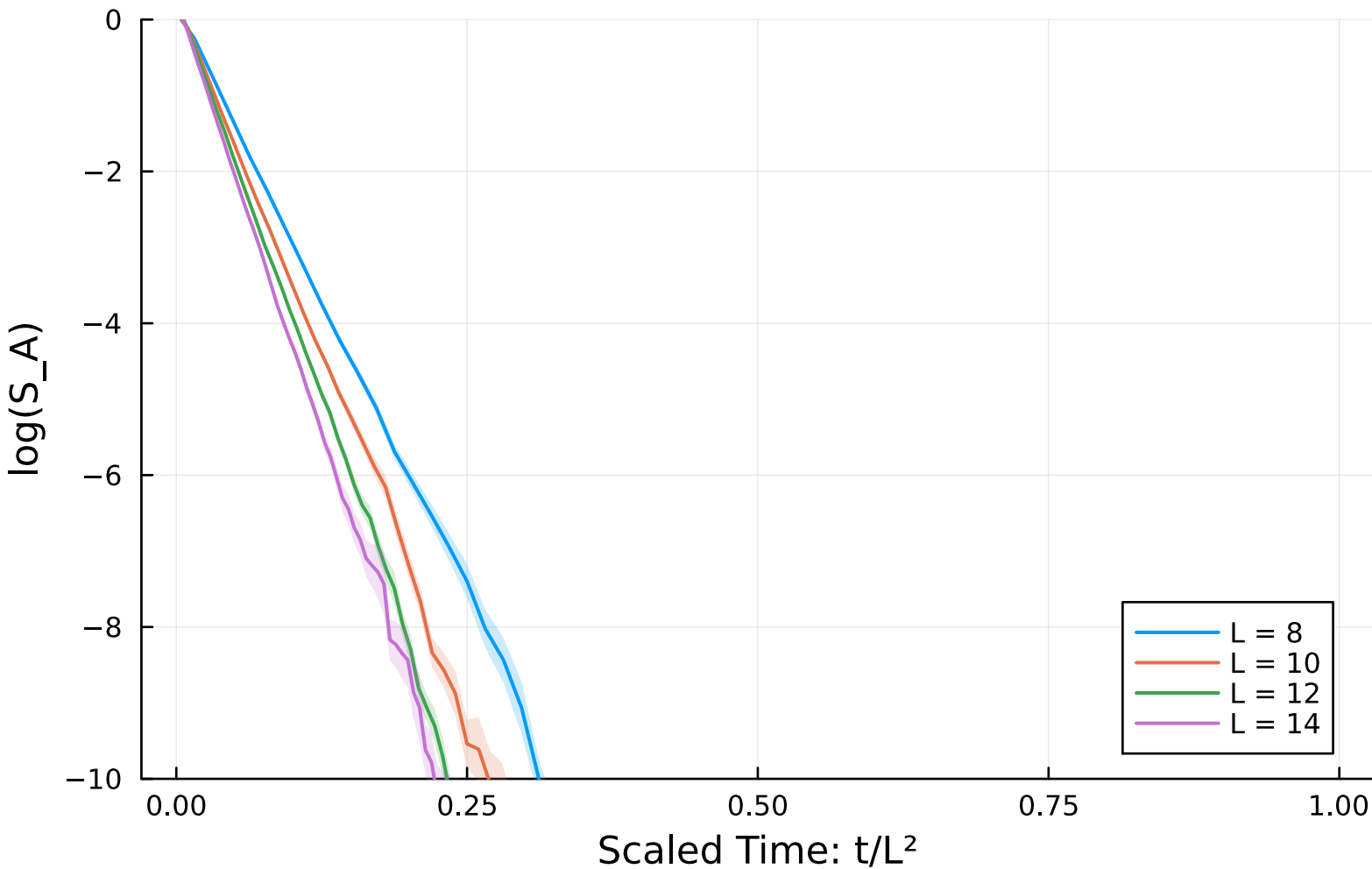
Scaled Log Entropy Evolution ( p = 0.633333 )
